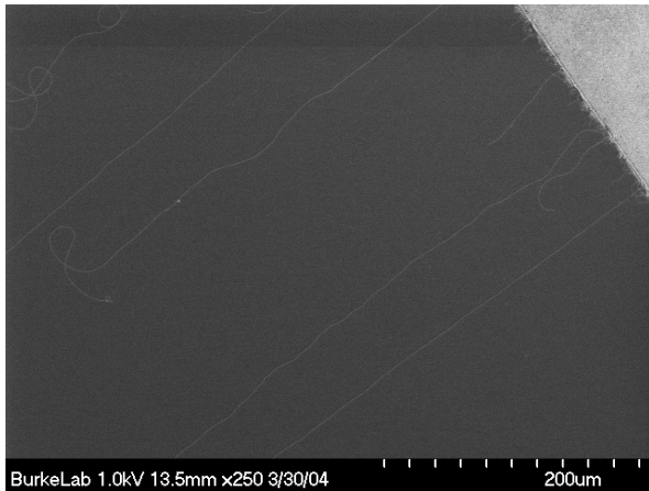
Figure 2: SEM image of arrayed, ultra-long single-walled nanotubes synthesized in our labs.
