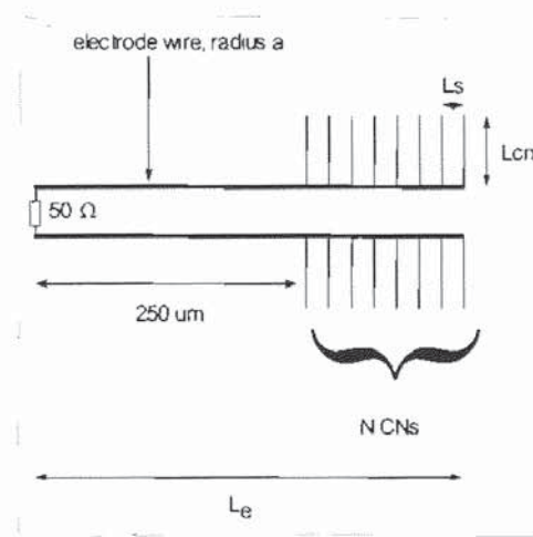
Fig. 10. Carbon nanotube antenna array geometry for simulation.
