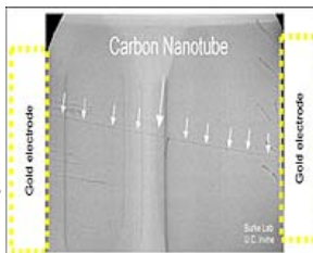
0.4 Electrically Contacted Carbon Nanotube. Image credit: Burke Lab/ UC Irvine.
